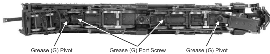
Figure: Grease points
