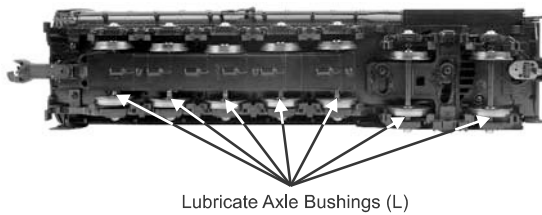
Figure: Lubrication Points on the Locomotive and Tender
